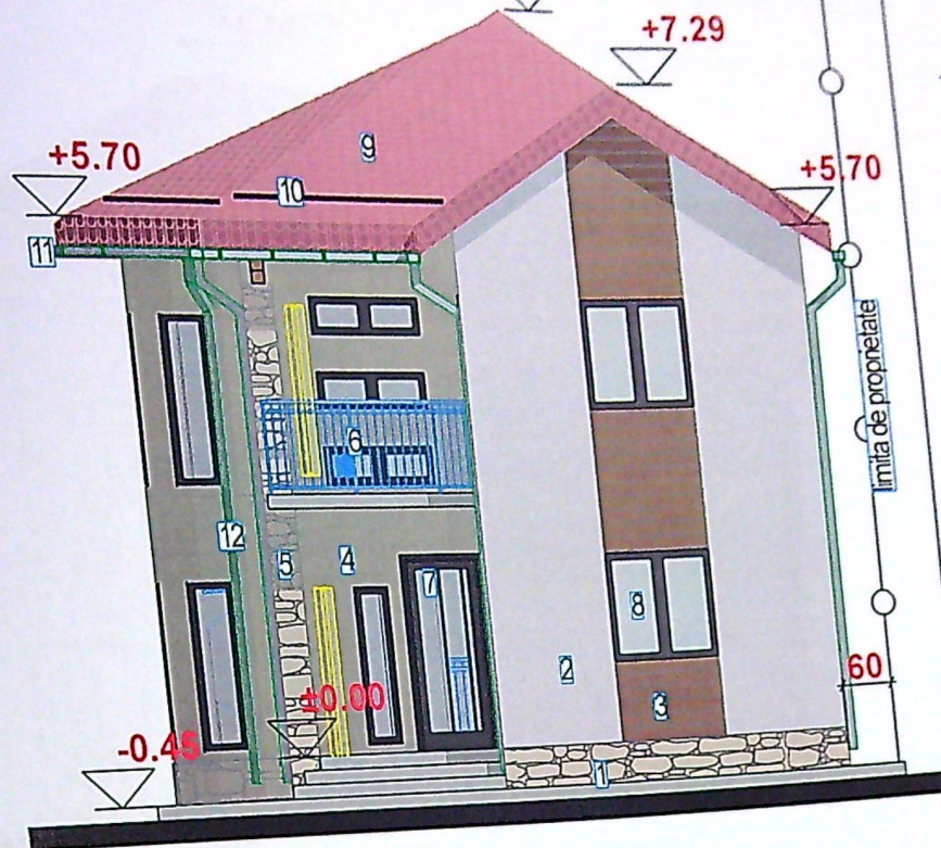
FATADA PRINCIPALA
